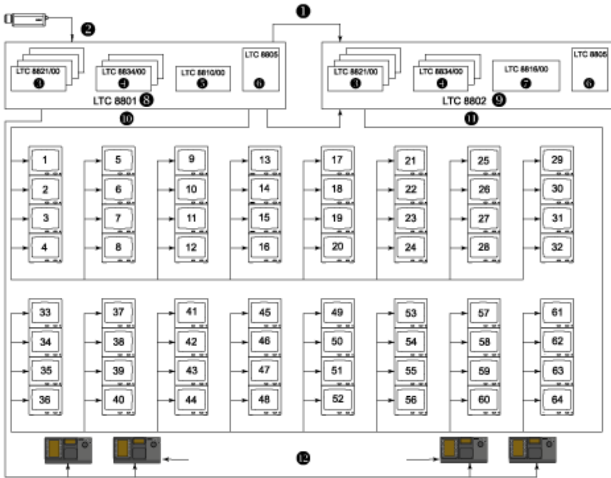
LTC 8800 Series Dual-bay System (256 Cameras by 64 Monitors)
