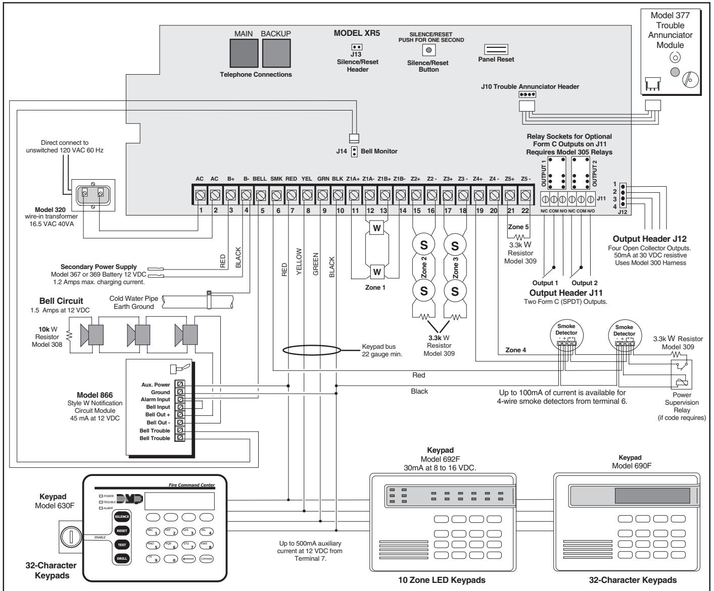
XR5FC System Configuration Diagram
